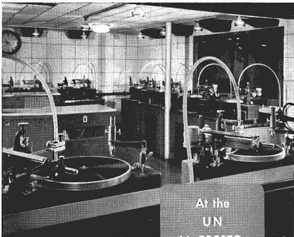
Ten Presto 8-D recorders in the United Nations' recording studio at Lake Success, Long Island, N.Y.
